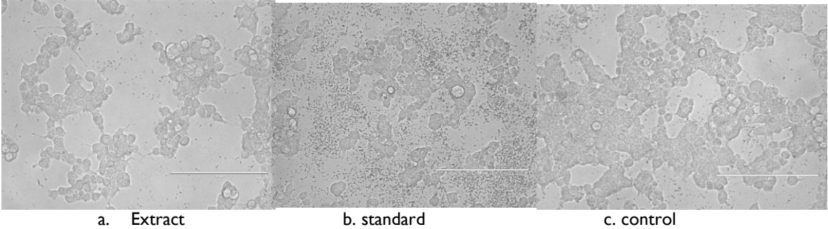
Fig. 3.a, 3.b, 3.c Microscopic images of cell line method
