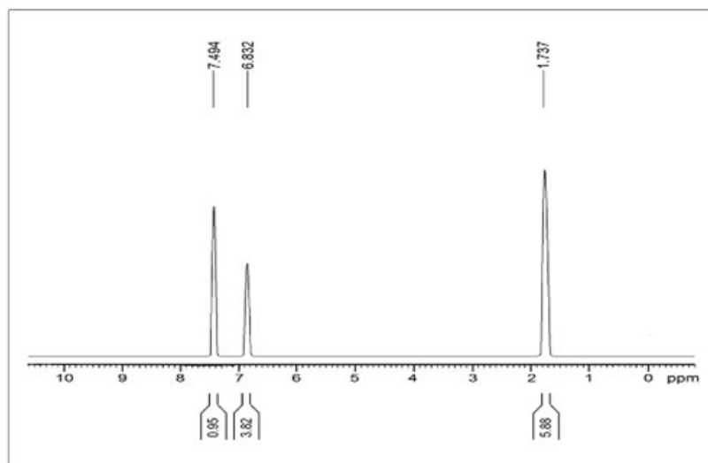
Figure 5 The ^1\text{H} NMR of metformin
