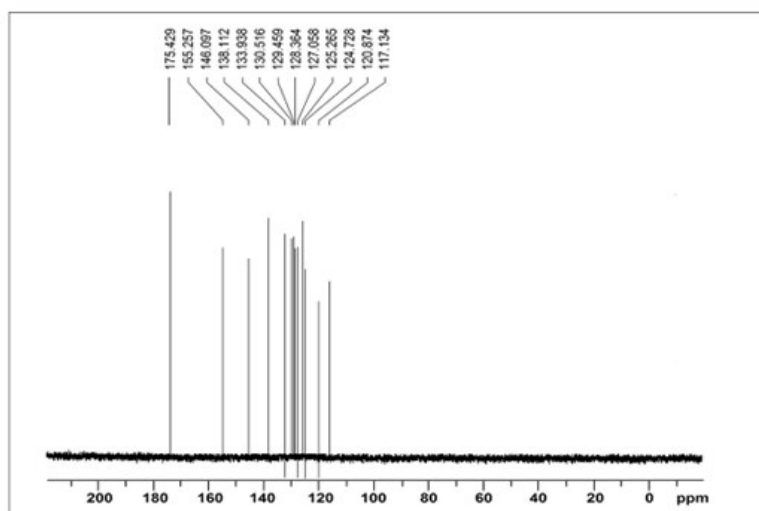
Figure 9 The ^{13}\text{C} NMR of 3-hydroxyflavone
