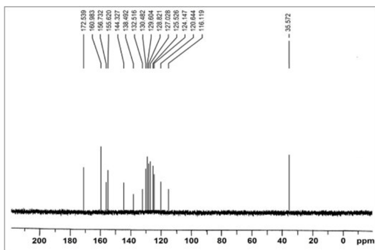
Figure 10 The ^{13}\text{C} NMR of metformin-3-hydroxyflavone complex
