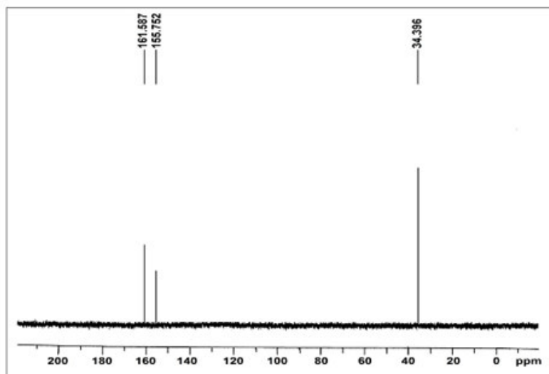
Figure 8 The ^{13}\text{C} NMR of metformin
